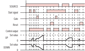
D : Signal OFF delay (Timer resets when power comes ON)
